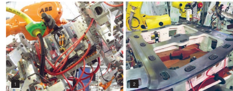
1 GVMAX vacuum pumps with protective cover on robot equipment
